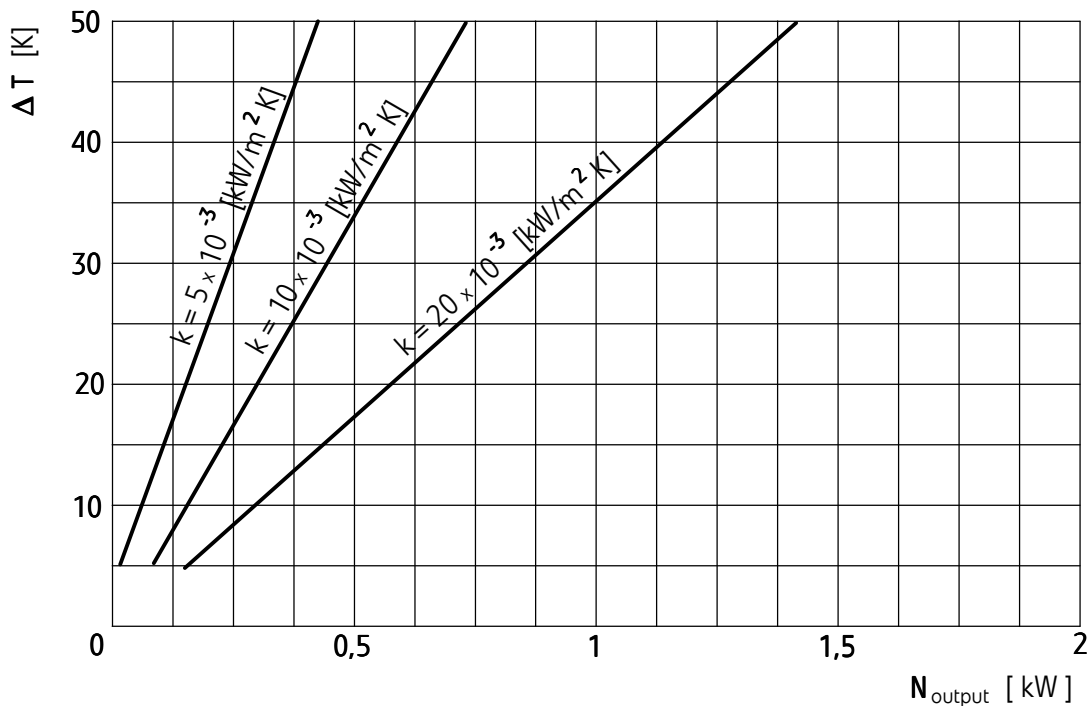
Thermal power output of the power pack tank UHJV100
